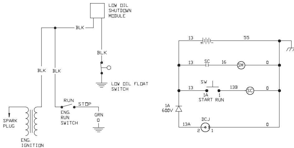
SCHEMATIC
